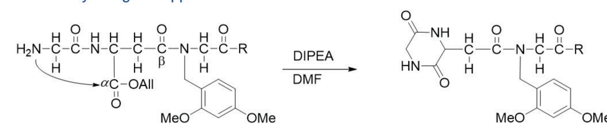
Scheme 2: On-resin formation of cyclo(-Gly-Asp)-Dmb-Gly-Ala-Lys(Boc)-Phe-NH 2 . Subsequent TFA cleavage from the resin/ deprotection of side chain and backbone protecting groups yielding the crude DKP reference
