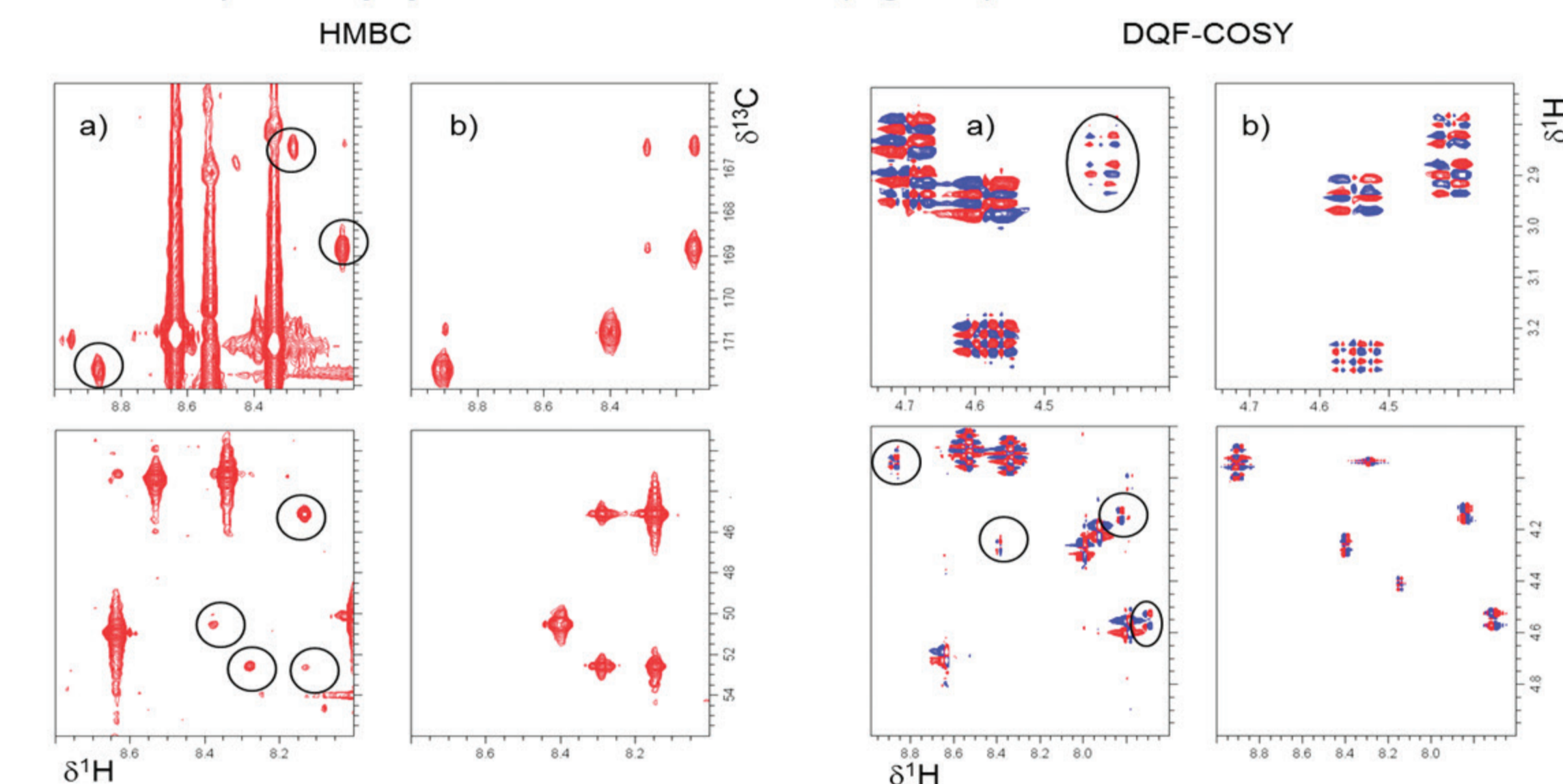
Figure 6: Enlarged regions of 1 H- 13 C HMBC and 1 H- 1 H DQF-COSY NMR spectra recorded in DMF-d 7 of a) crude native peptide with indication of residual resonances assignable to the DKP by-product and b) synthesized purified DKP reference.
